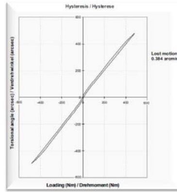
Lineer histerezis eğrisi
